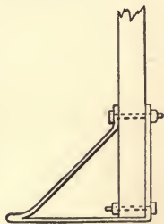
FIG. 8.—GRADE-ROD.
